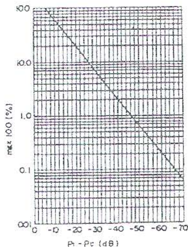
Fig. 6-3 AM Wave Modulation Factor and Sideband dB Display Level
