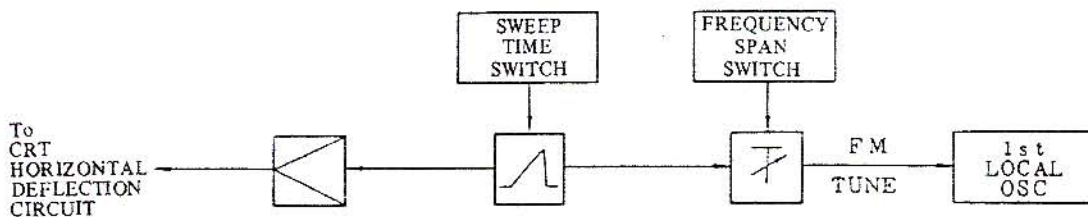
Fig. 3-5 MS610A Sawtooth Generator and Local Oscillator Control Circuit
