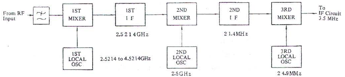
Fig. 3-2 MS610A Frequency Conversion Circuit
