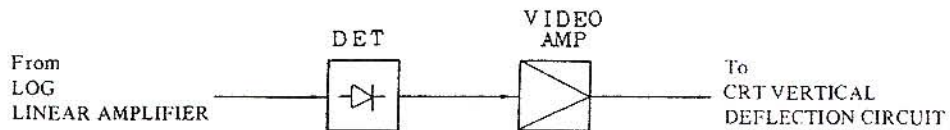
Fig. 3-4 MS610A Detection and Video Circuits
