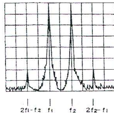
Fig. 6-8 Inter Modulated Wave Spectrum Display
