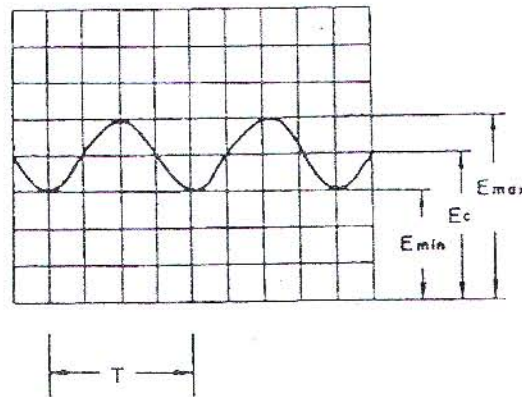
Fig. 6-4 AM Wave Time Domain Display Example
