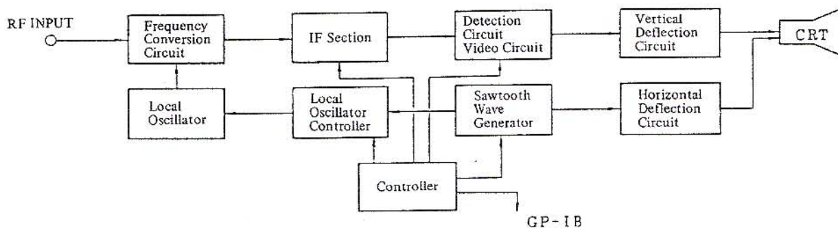
Fig. 3-1 MS610A Block Diagram
